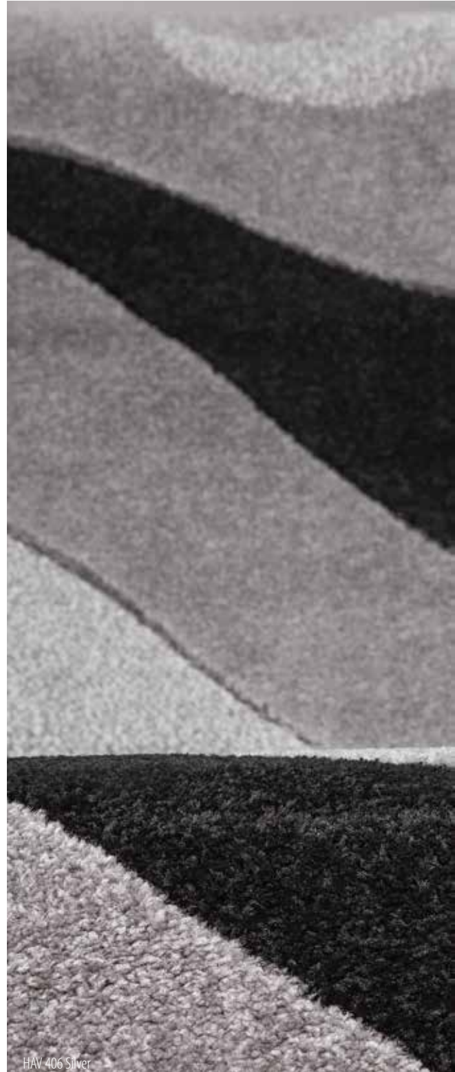
HAV 406 Coffee
